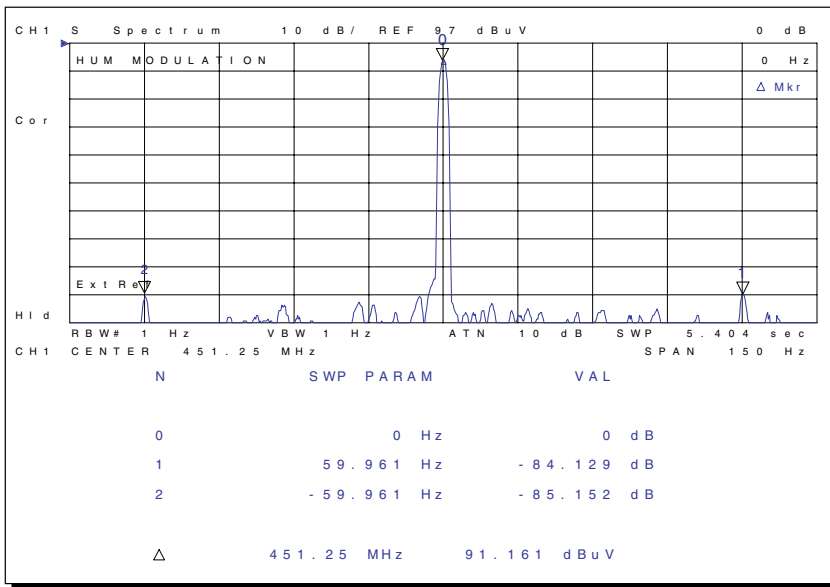
Figure 24. Example of Hum Modulation Measurement Results
