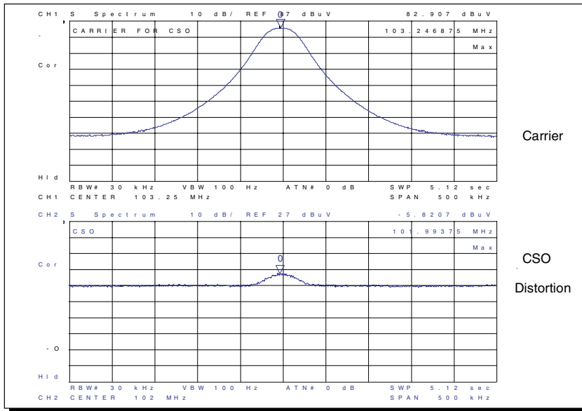
Figure 18. CSO Measurement Results Using the Agilent 4396B
