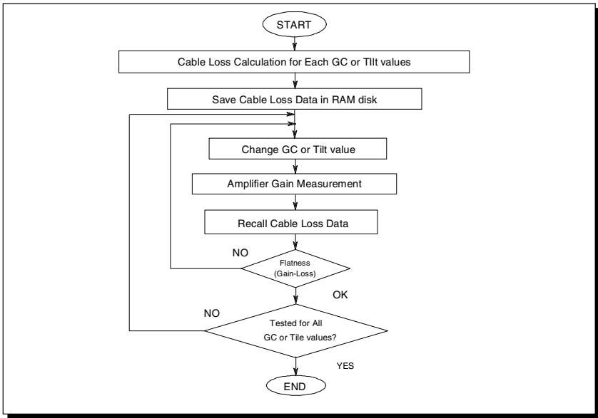
Figure 11. Agilent 4396B IBASIC Program Flowchart
