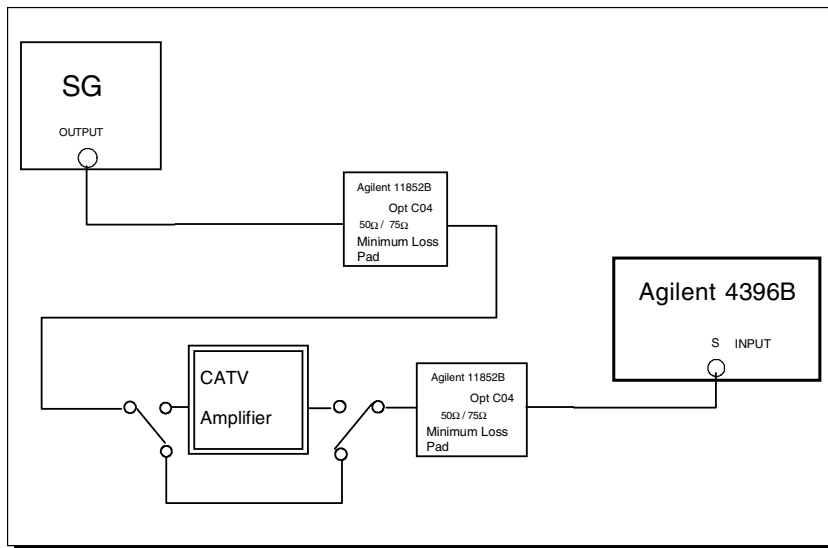
Figure 23. Example of Measurement System Configuration for Hum Modulation
