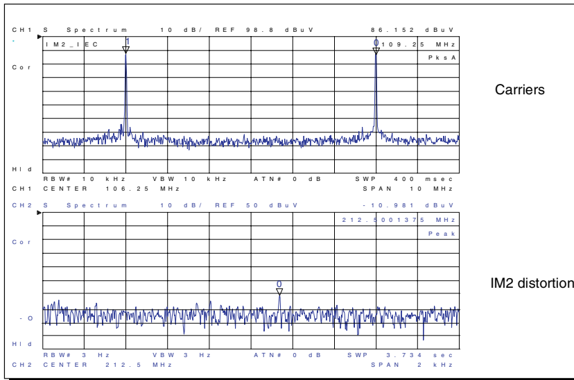
Figure 22. Example of Inter-Modulation Distortion Measurement Results Using the Agilent 4396B
