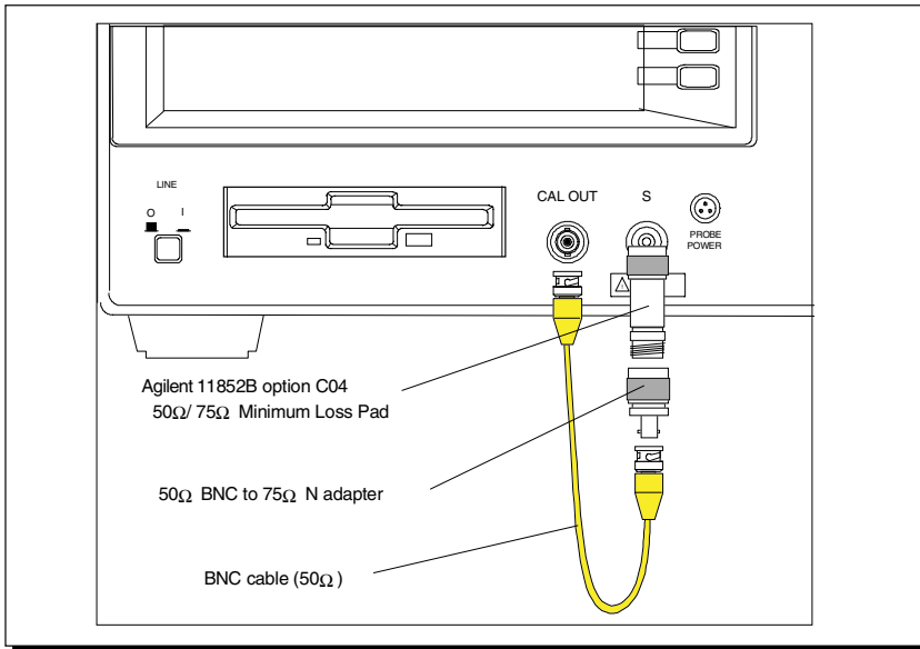
Figure 14. Reference Level Calibration of the Agilent 4396B for Measurement of Amplifier with 75Ω Impedance
