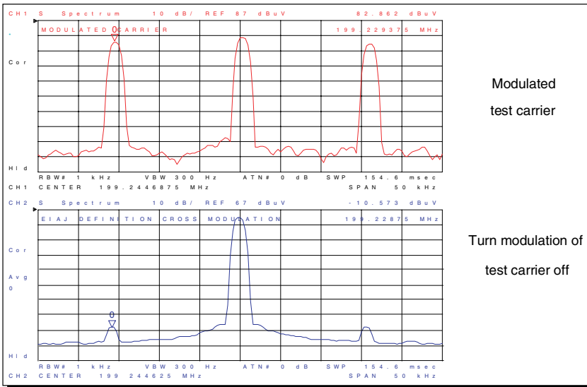
Figure 19. Example of Cross Modulation Distortion Measurement Results Using the Agilent 4396B (per EIAJ ET-2301 Standard)
