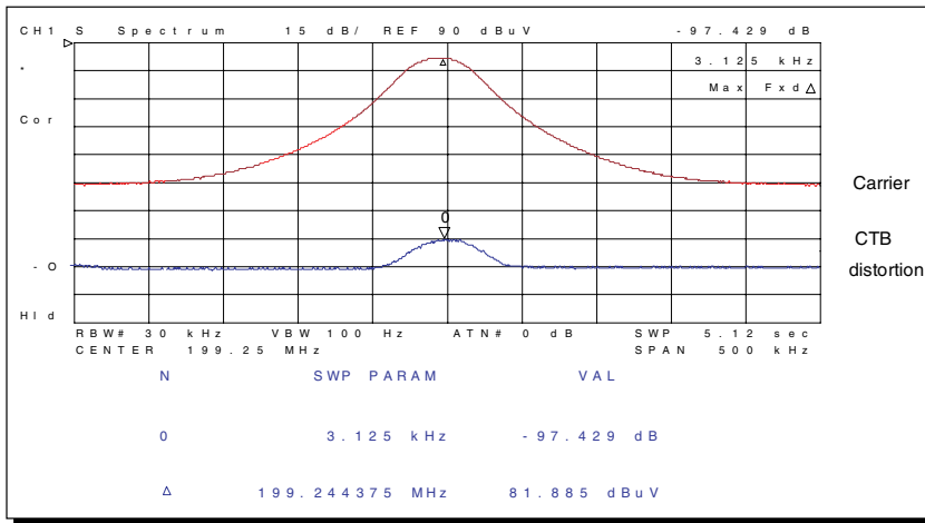
Figure 17. CTB Measurement Results Using the Agilent 4396B
