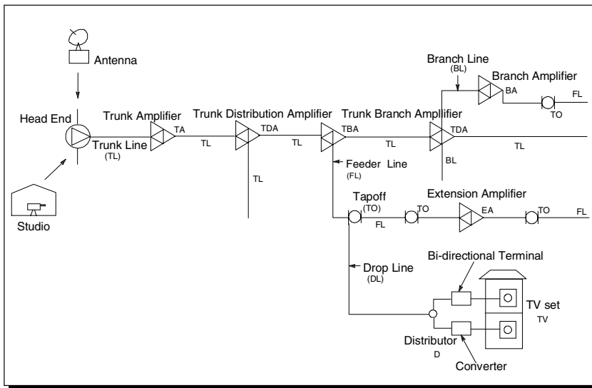
Figure 1. CATV System Configuration
