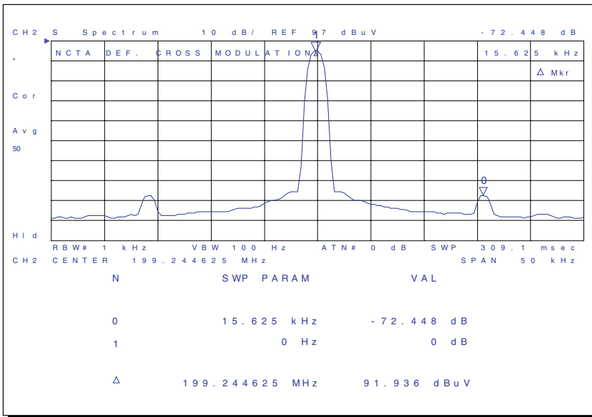
Figure 20. Example of Cross Modulation Distortion Measurement Results Using the Agilent 4396B (per NCTA Standard)
