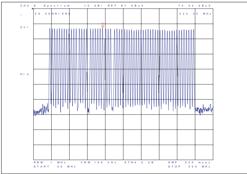
Figure 16. Carrier Output from Multi-Channel Signal Generator
