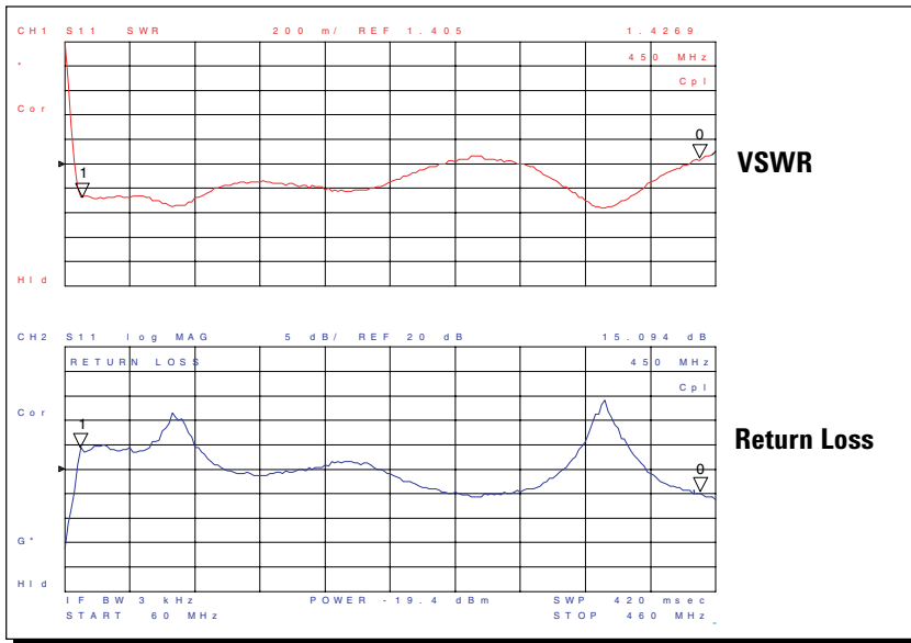
Figure 13. CATV Amplifier Reflection Characteristic Measurement Results
