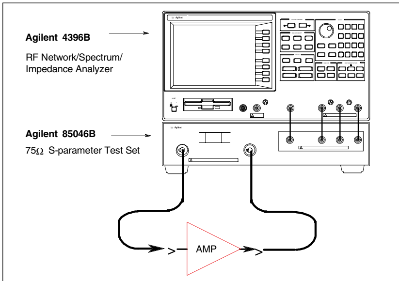
Figure 2. Example of Network Measurement System Configuration
