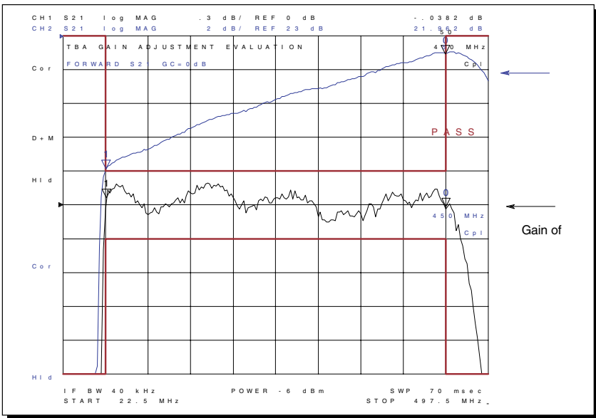
Figure 12. Example of Real Time Pass/Fail Test Results for CATV Amplifier Gain Control Capability Using the Agilent 4396B
