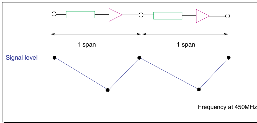
Figure 6. Cable Loss per Span
