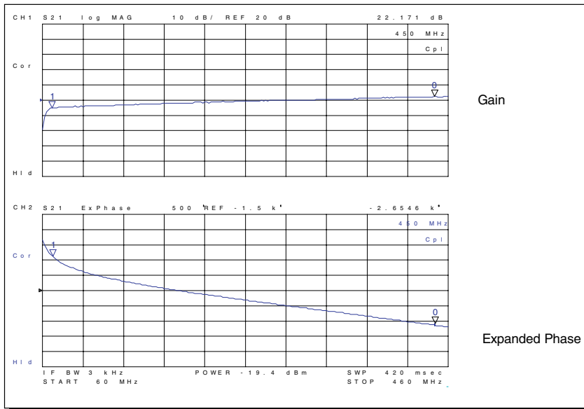
Figure 3. Example of Amplitude-Expanded Phase Measurement Results
