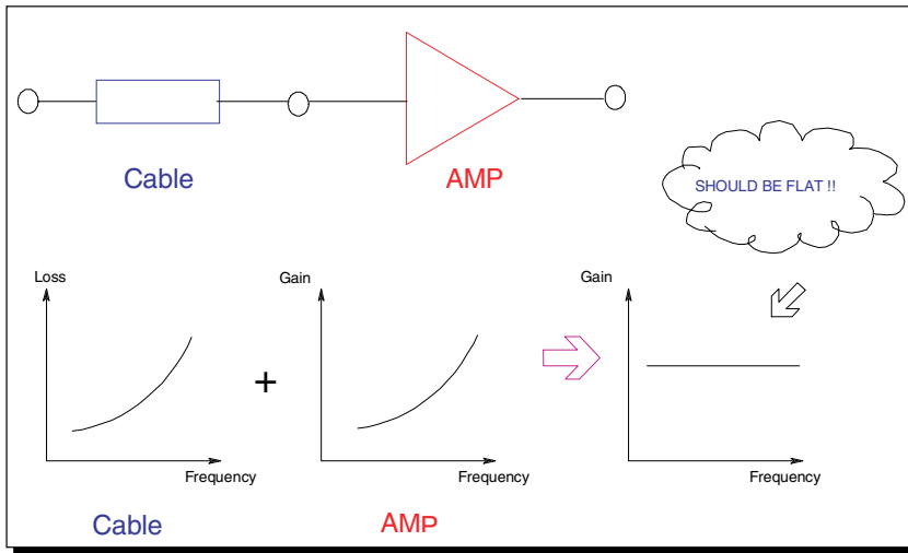
Figure 5. Transmission System Composed of Cable and Amplifier
